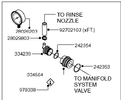
RINSE SYSTEM- MANIFOLD SYSTEM
