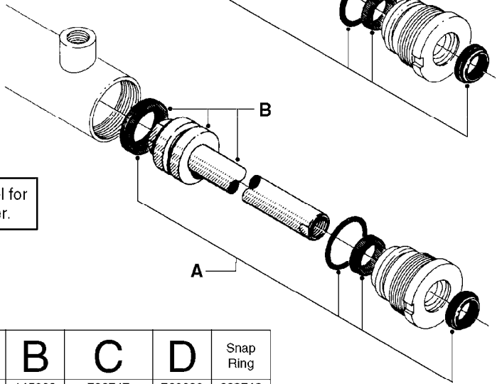
SINGLE-ACTING CYLINDER
