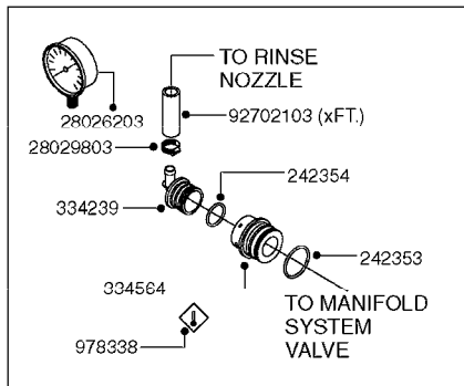
RINSE SYSTEM- MANIFOLD SYSTEM
