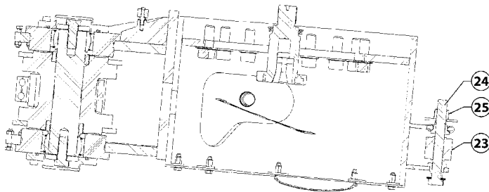
CROSS SECTION H-H
