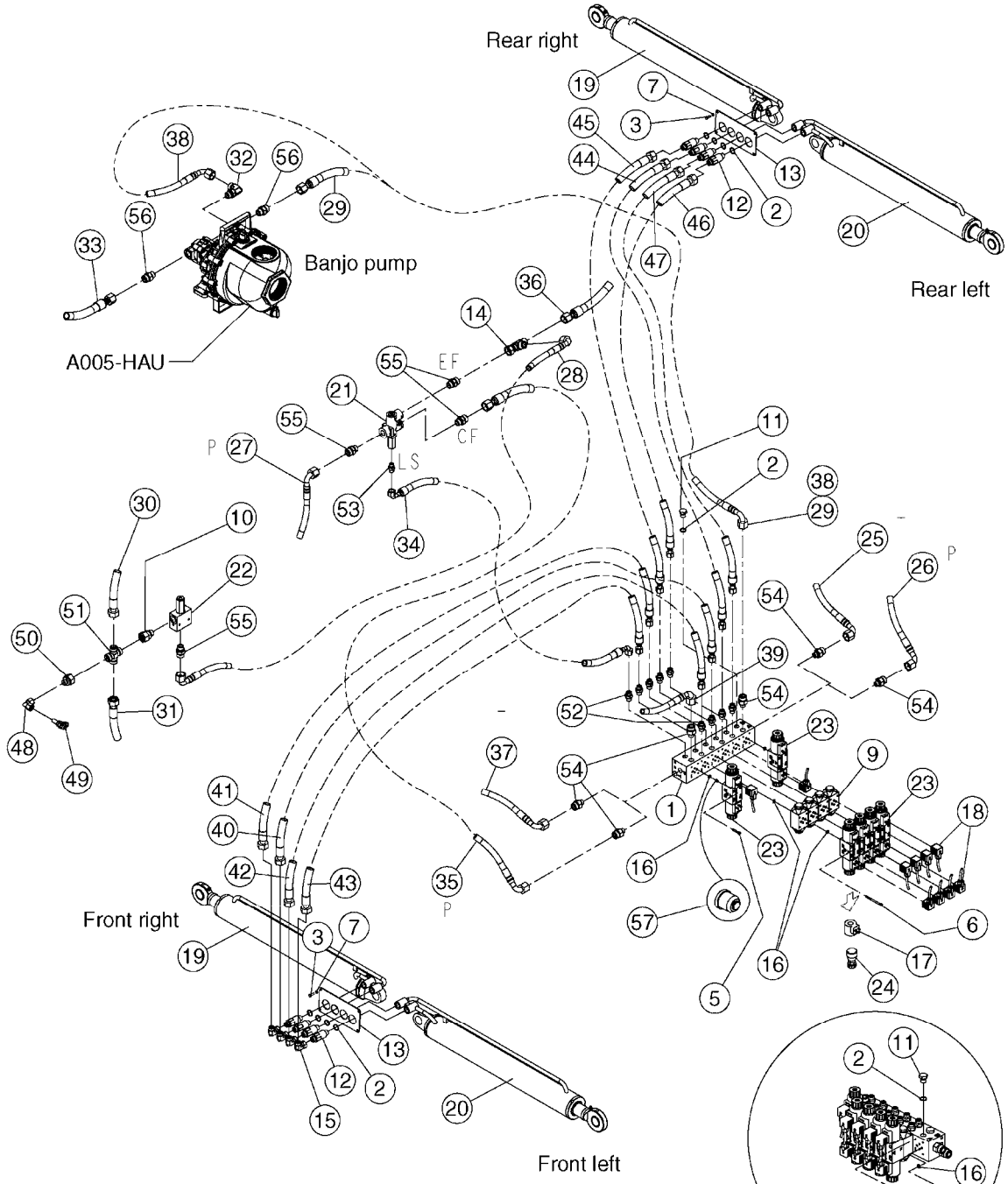
Assembly without Banjo pump
