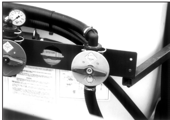
Fig. 62 Agitation Bypass Valve
