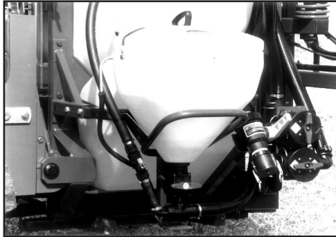
Fig. 51 Chemical Filler Installed
