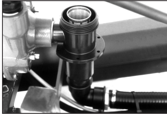
Fig. 61 Suction Filter
