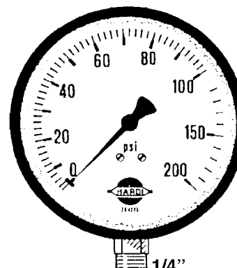
1/4" 28026103 0-100-200 psi STAINLESS 4" GAUGE
