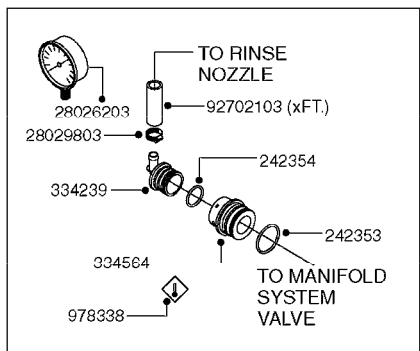
RINSE SYSTEM- MANIFOLD SYSTEM
