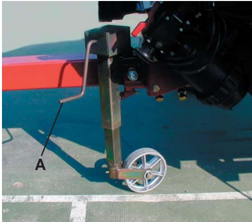
Sprayer unattached
