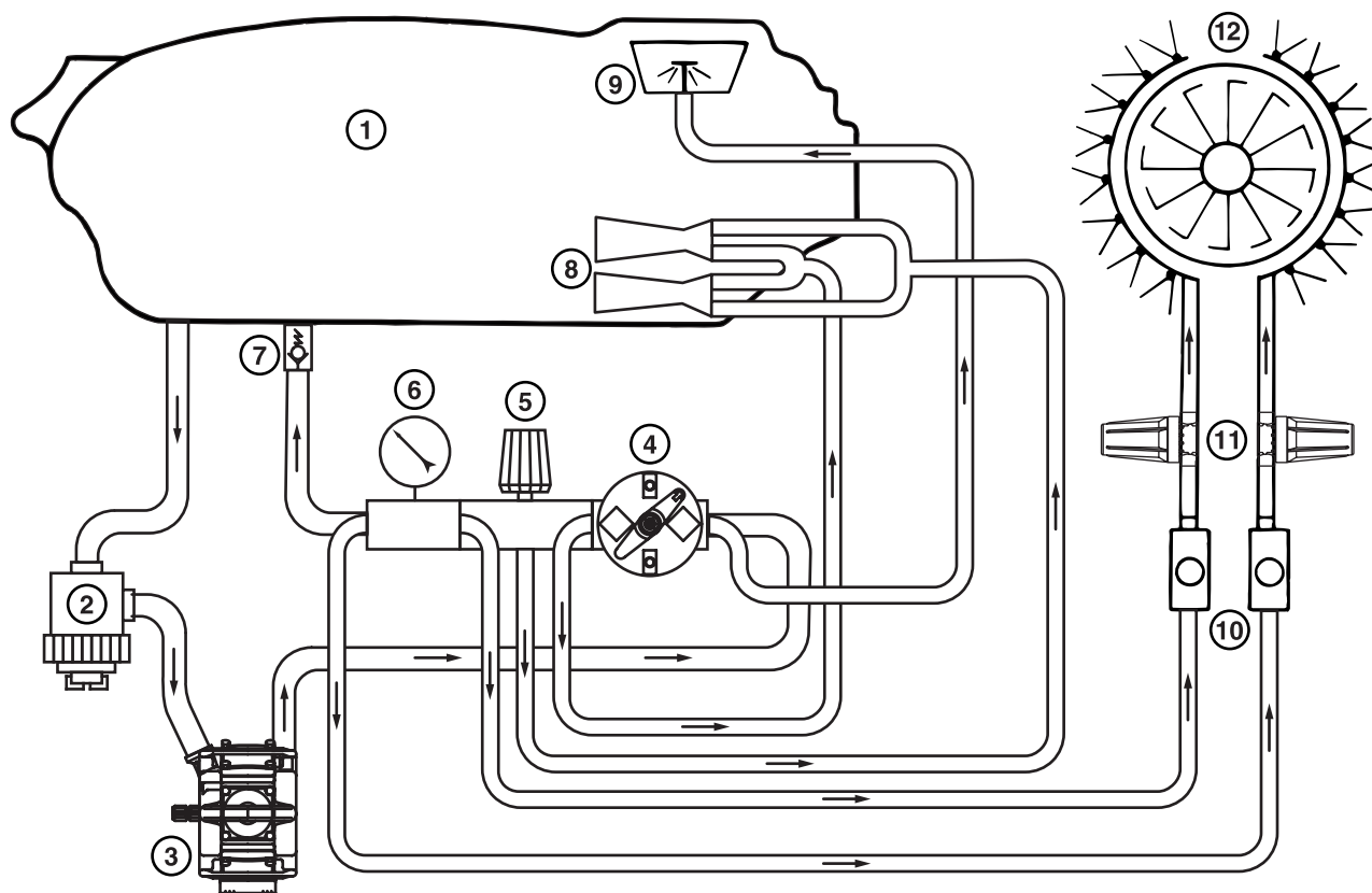
mercury 600 - HC/2
