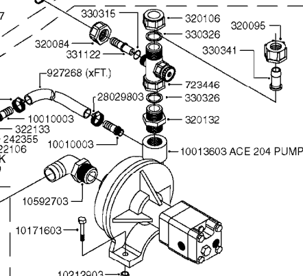
PUMP KIT 10547303
